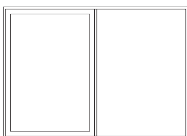
2-FAGS
